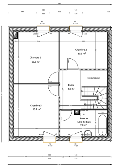
PLAN R+1
